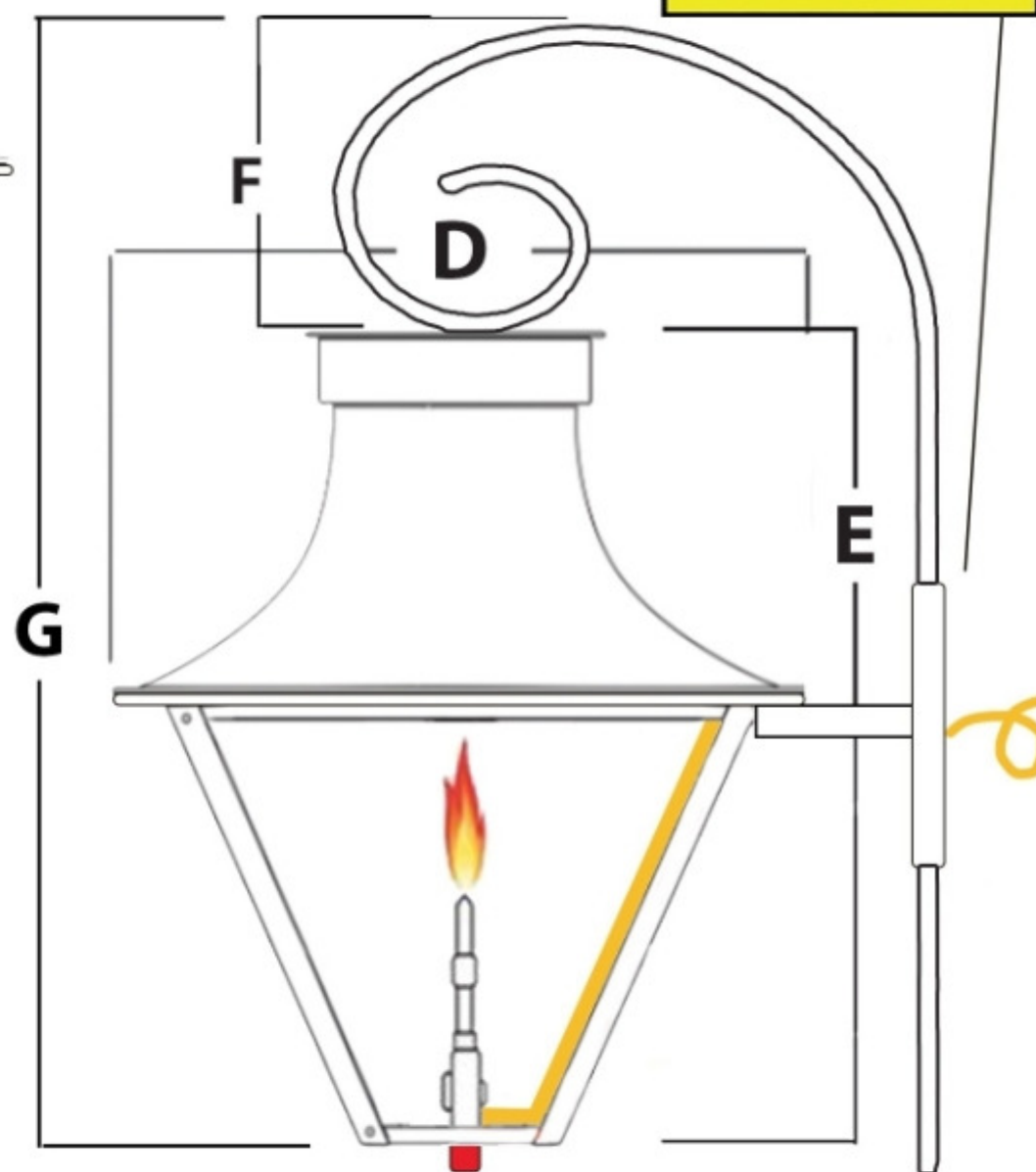
Side View
