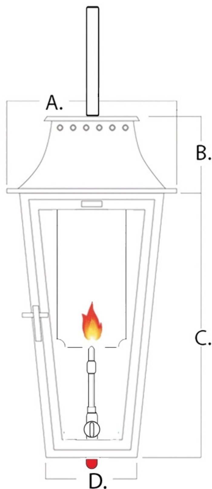
Front View
