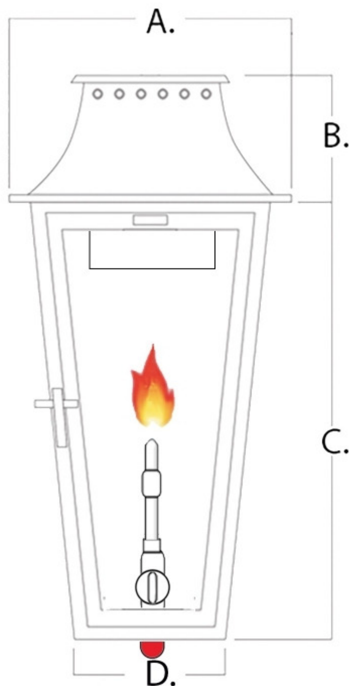
Front View
