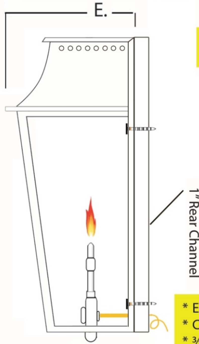
SIDE VIEW
