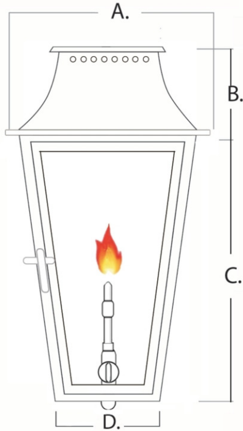
FRONT VIEW
