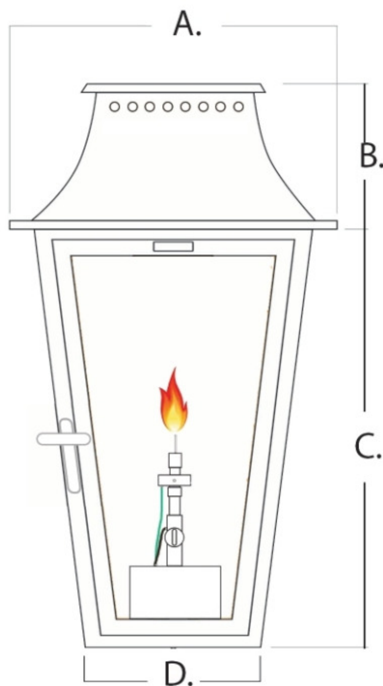
FRONT VIEW
