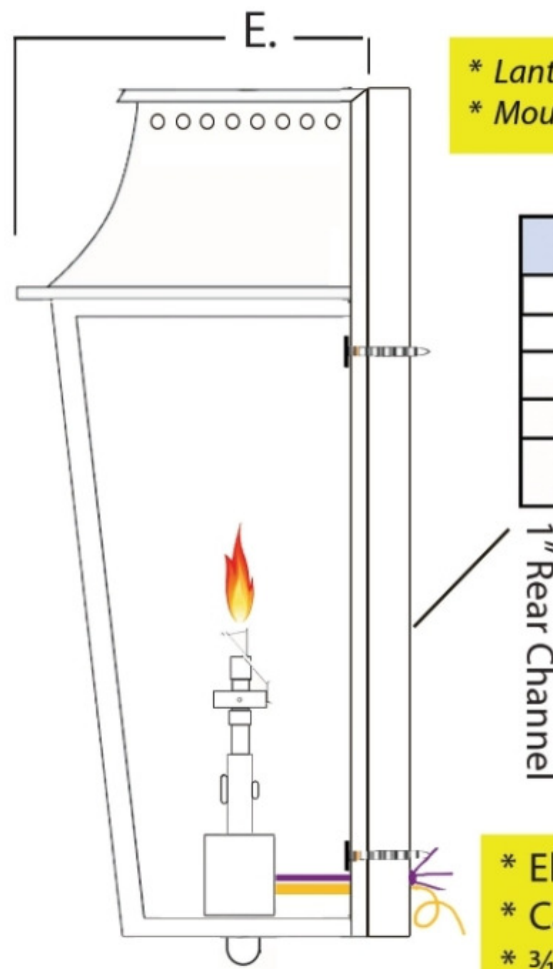
SIDE VIEW
