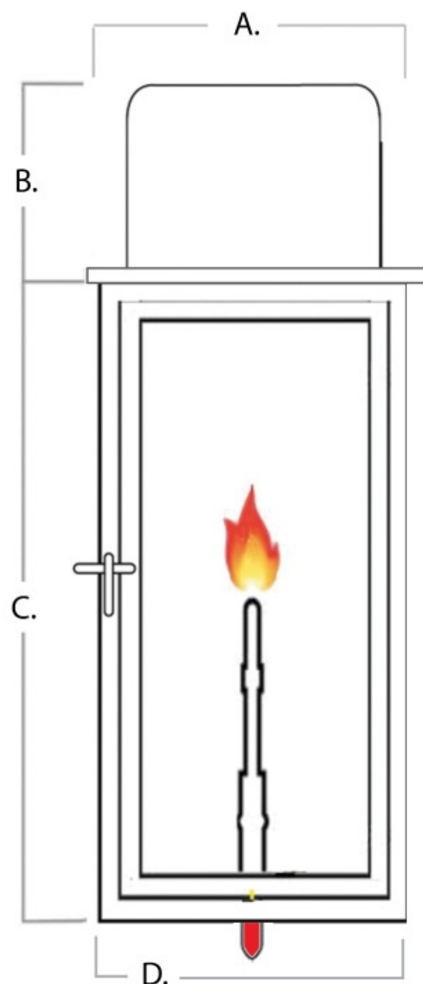
Front View
