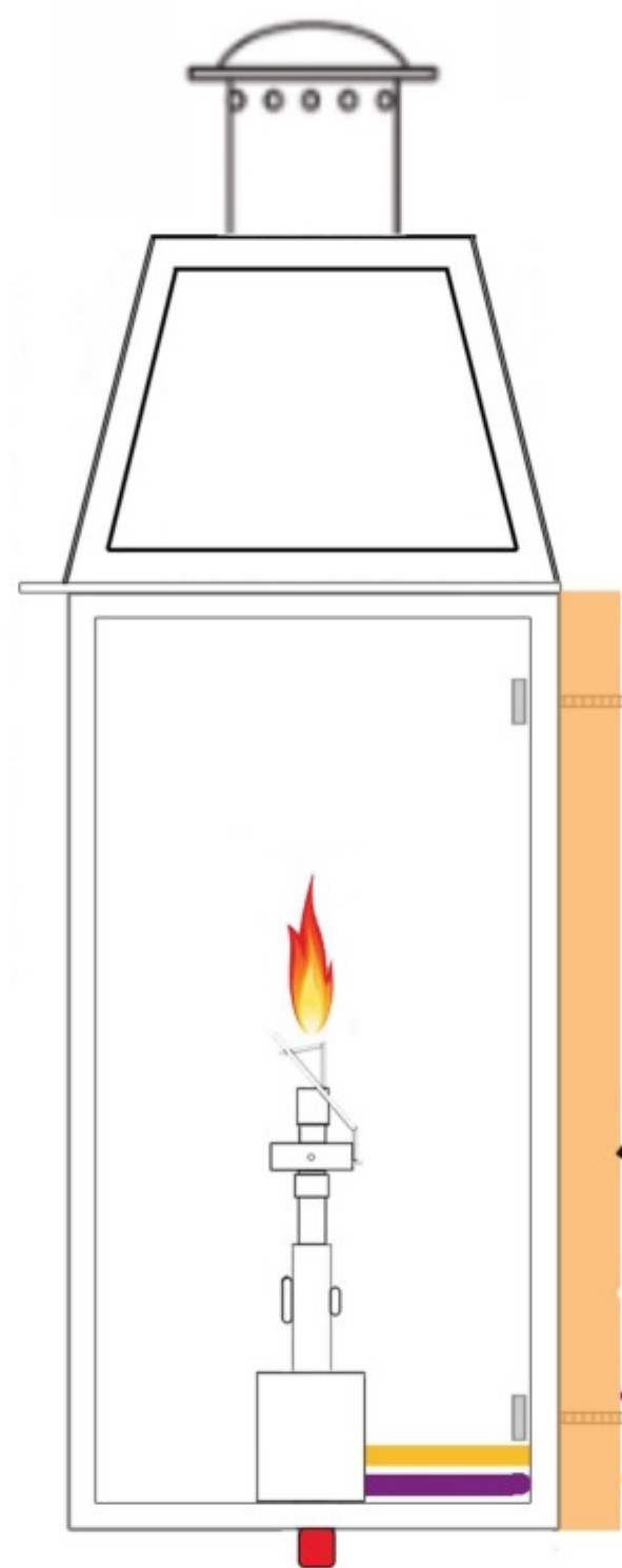
SIDE VIEW
