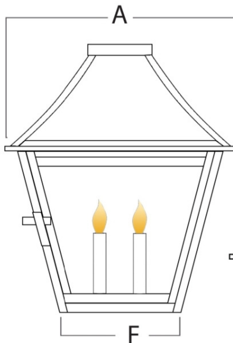
Front View
