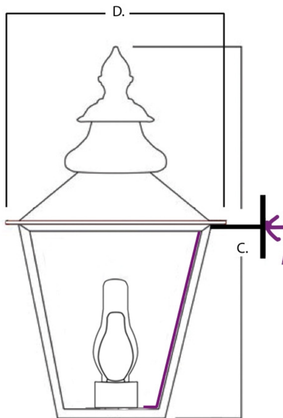
Side View
