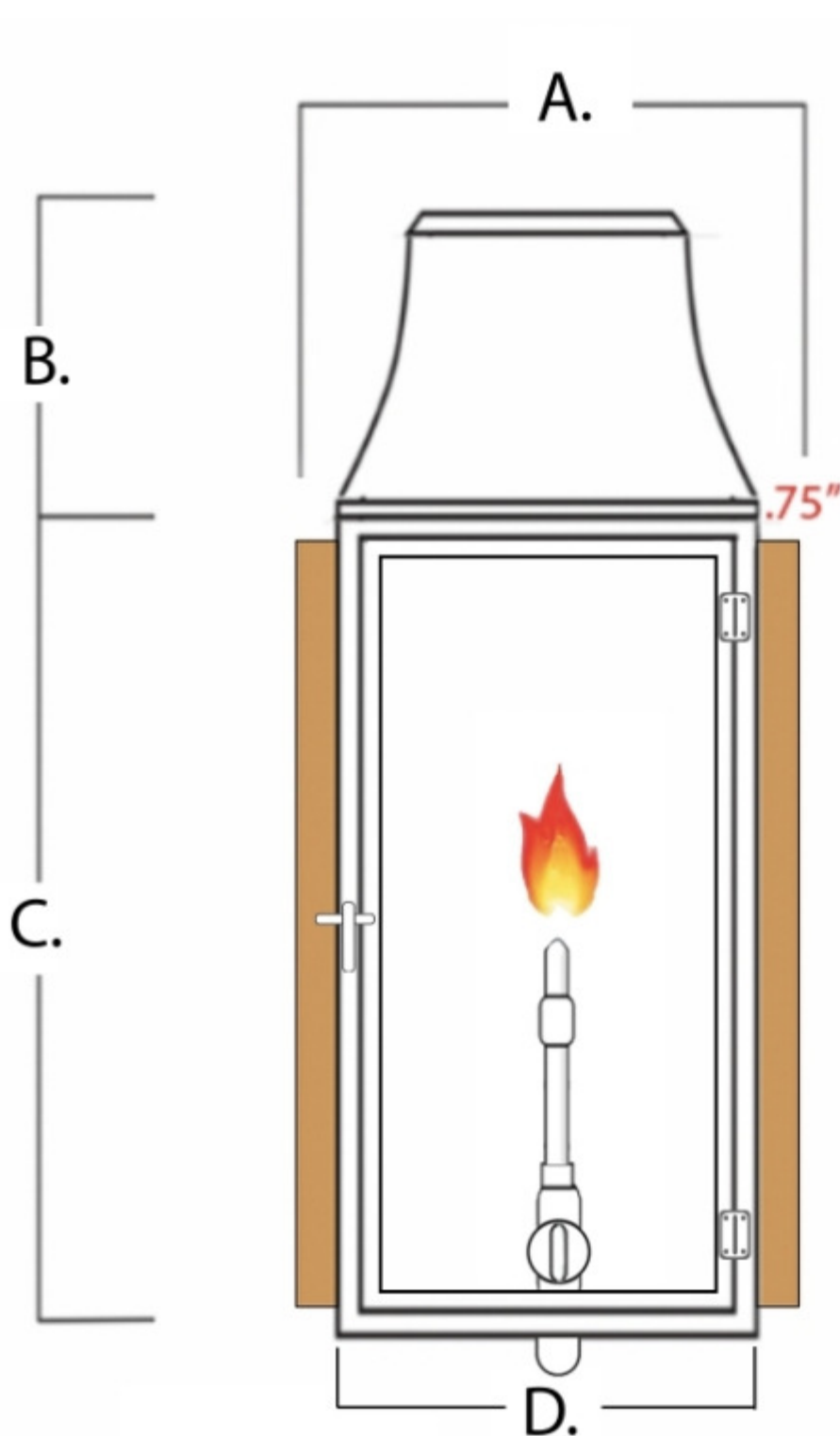
Front View
